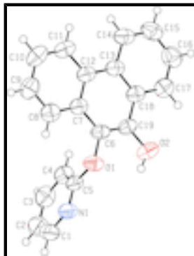
Fig. 1. The molecular structure of the title compound with the atom numbering scheme. Displacement ellipsoids are drawn at the 50% probability level. H atoms are presented as a small spheres of arbitrary radius.
